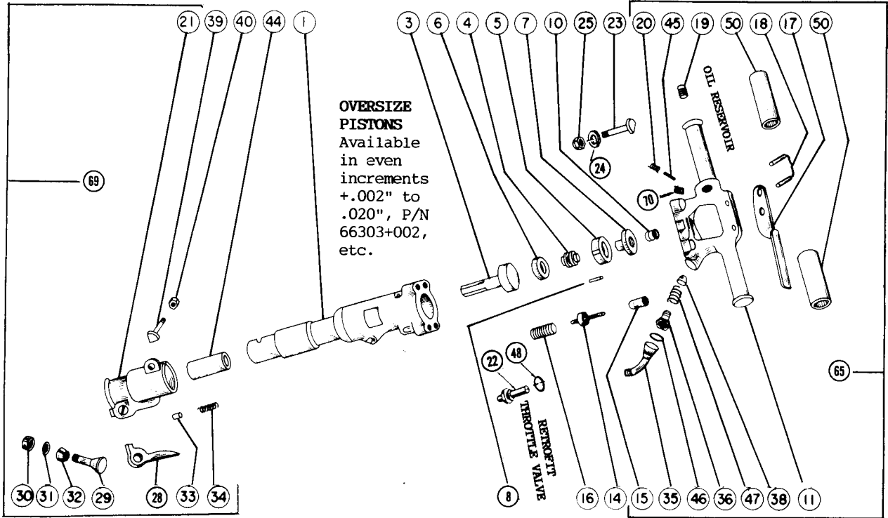
MODEL 4014 - 7/8" x 3-1/4" HEX CHUCK MODEL 4015 - 1" x 4-1/4" HEX CHUCK
